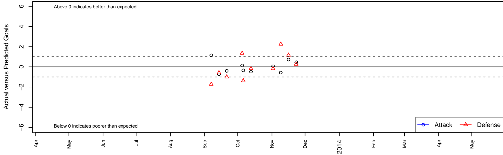
Diablo FC B00 Dots are actual minus expected GF (blue circles) and GA (red triangles). Blue line is smoothed change in attack strength. Red is smoothed change in defense strength.
